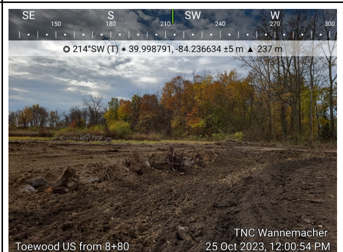
Photograph 4: Toewood revetment along south bank, upstream of Sta 8+80.
